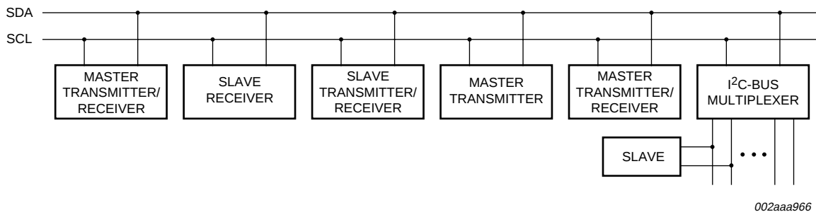
Fig 17. System configuration
